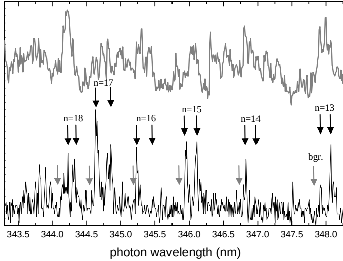
Figure 4.9: Predissociation scan of v = 1 Rydberg states (black spectrum) versus autoionisation scan (grey spectrum). The branching ratios are measured at 10 photon wavelengths corresponding to R = N_c = 1 and R = N_c = 3 transitions. The background is measured at photon wavelengths indicated by the grey arrows.
