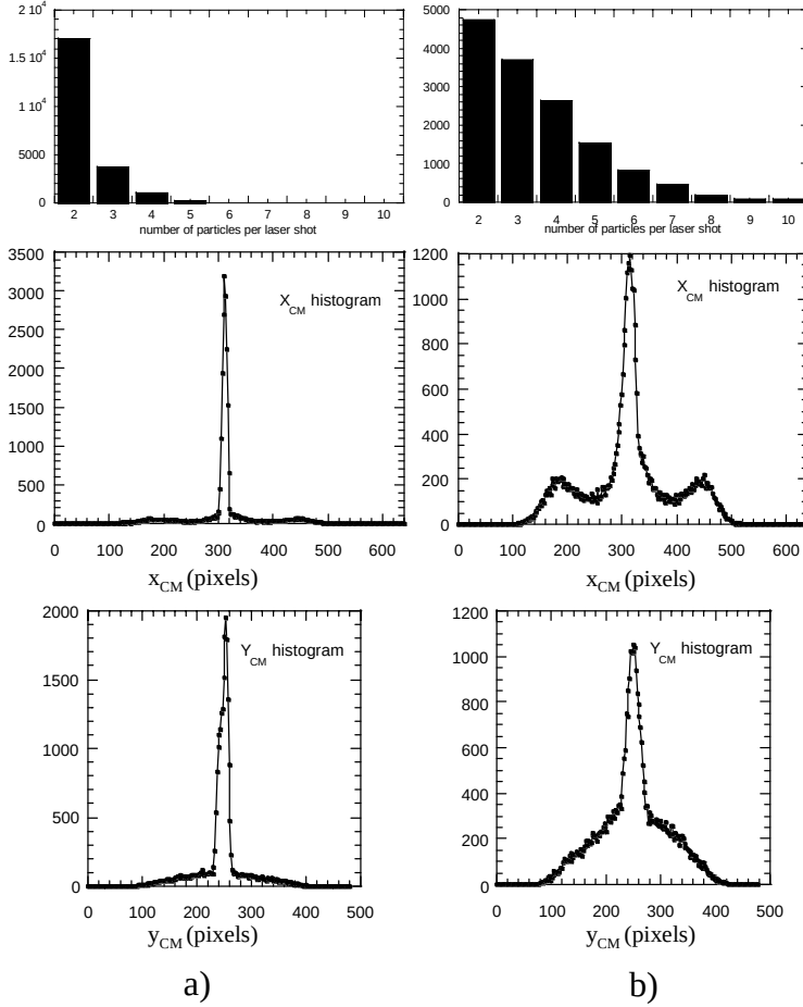
Figure 3.5: Centre-of-mass determination for two different data sets: a) low ion beam intensity; b) high ion beam intensity. The position histograms of the centre-of-mass for each combination of NO and O^- particles are shown. The fragments resulting from the same molecule appear in the central peaks.
