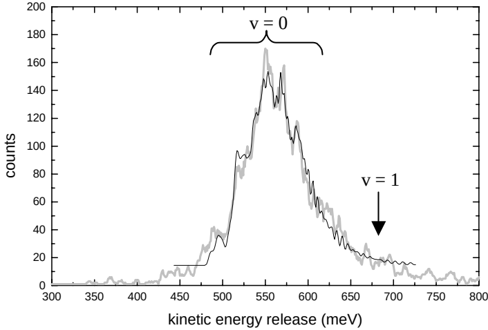
Figure 5.5: The KER spectrum (thick grey curve) shows a broad but structural feature around 550 meV associated with transitions from O_2^- (X^2\Pi_{g,\Omega}) ( \Omega = 3/2, 1/2 ) ( v=0 ) states and leading to the O(^3P_{2,1,0}) + O^-(^2P_{3/2,1/2}) limits. No photofragments starting from O_2^- (v=1) are observed. The fit (thin black curve) is a linear superposition of 12 possible fine-structure transitions and the background line. The results of the fit are presented in Table II.
