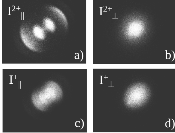
Figure 2.3: Experimental images recorded using femtosecond dissociative ionization of molecular iodine. The four situations shown are (a) I_2^+ , polarisation parallel; (b) I_2^+ , polarisation perpendicular; (c) I^+ , polarisation parallel; (d) I^+ , polarisation perpendicular.
